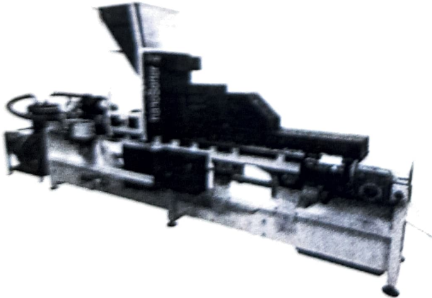
nanoSorter Shuka Neo Cashew Grading Machine
